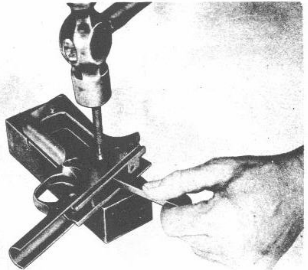
Figure 159. Riveting front sight on slide.
